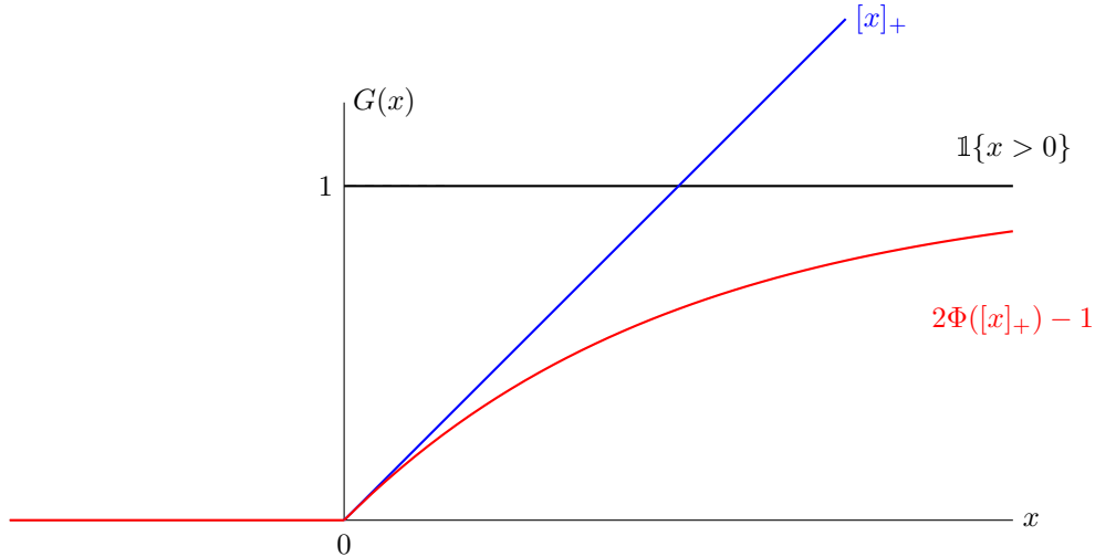
Figure 6: G(\cdot) Functions
